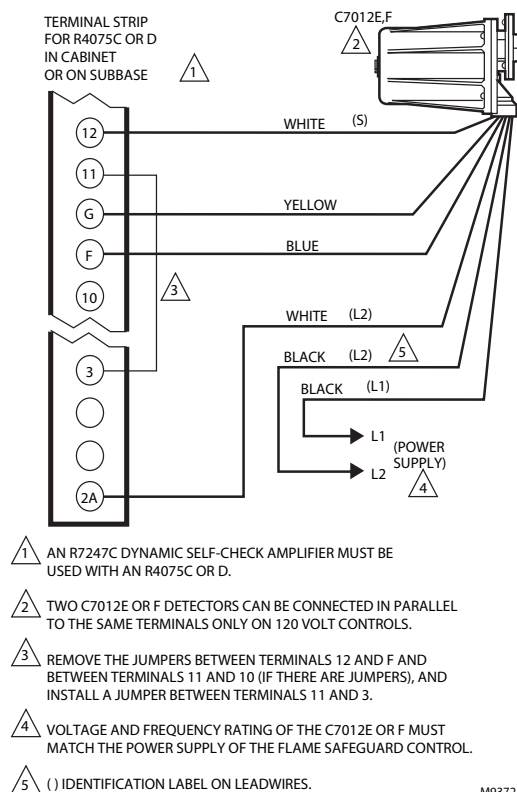
Fig. 11. Wiring diagram for C7012E or F Detectors with R4075C or D (currently obsolete) Flame Safeguard Controls.
